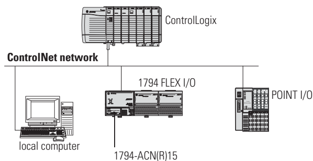
Figure 2 - ControlNet Communication
