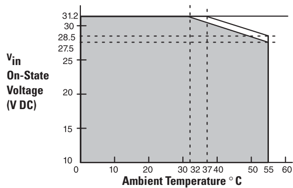
1794-OB16P Derating Curve
