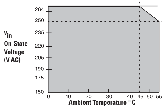
1794-IM8 Derating Curve
